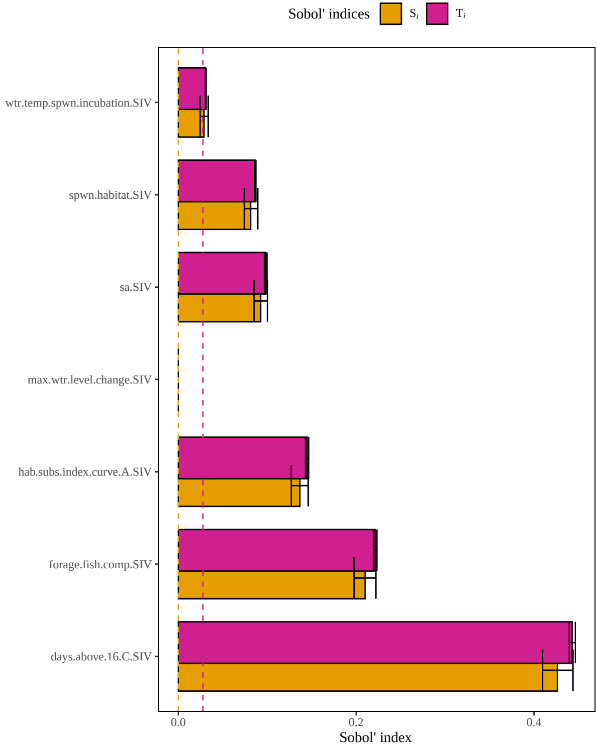
Figure 5. Results of a sensitivity analysis for the whitebassLacCurveASubIndex model based on a geometric mean structure. Dashed lines represent baseline numerical approximation error for S_i and T_i ( i.e. , dummy variables).
