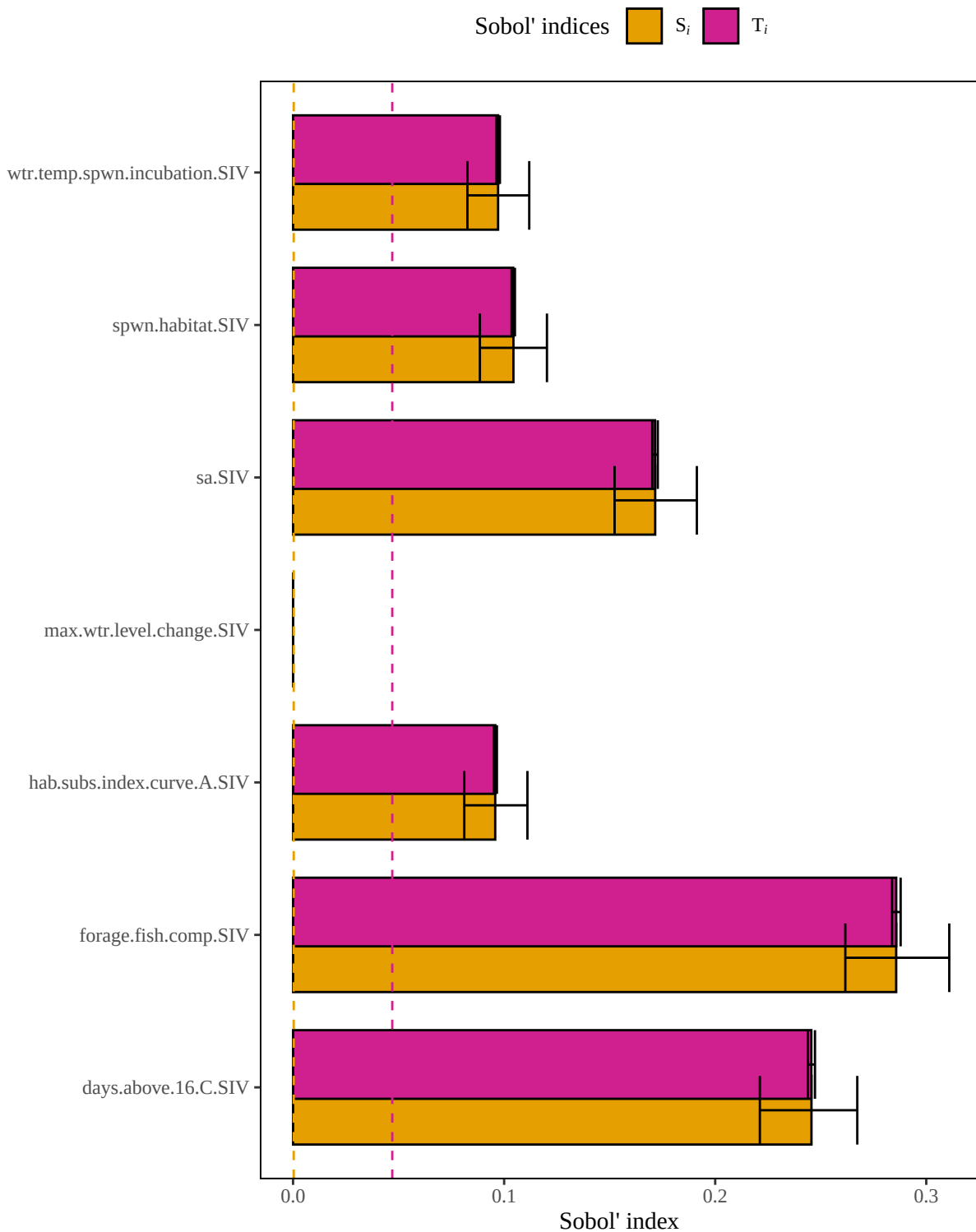
Figure 4. Results of a sensitivity analysis for the whitebassLacCurveASubsIndex model based on an arithmetic mean structure. Dashed lines represent baseline numerical approximation error for S_i and T_i ( i.e. , dummy variables).
