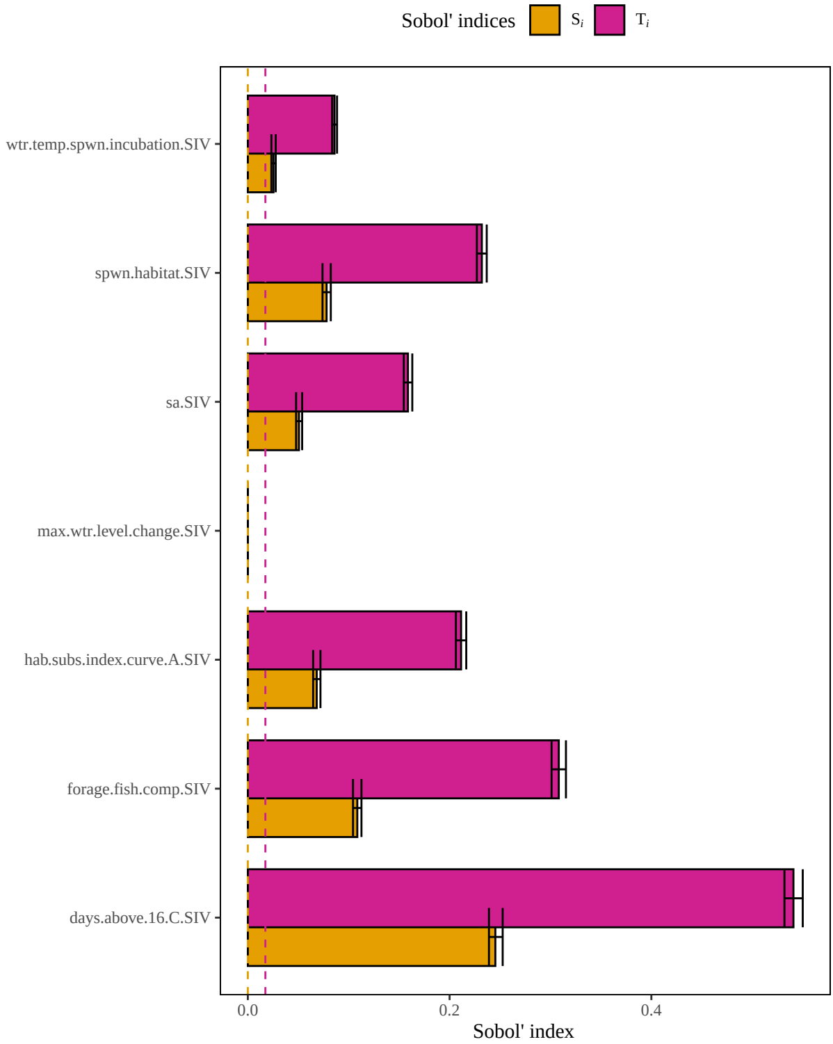
Figure 7. Results of a sensitivity analysis for the whitebassLacCurveASubsIndex model based on a multiplicative mean structure. Dashed lines represent baseline numerical approximation error for S_i and T_i ( i.e. , dummy variables).
